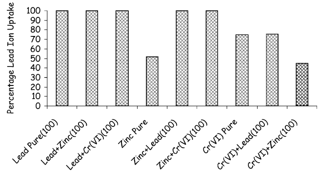
Fig. 5. Effect of multi-component system on metal removal.
