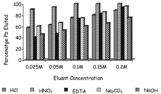
Fig. 6. Elution tests.
